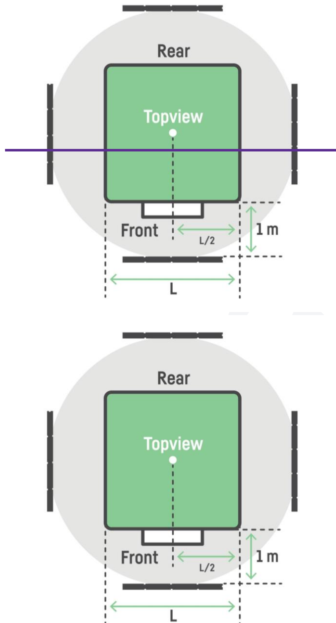
Figure alternating electric fields 1. Measurement geometry for band II.
