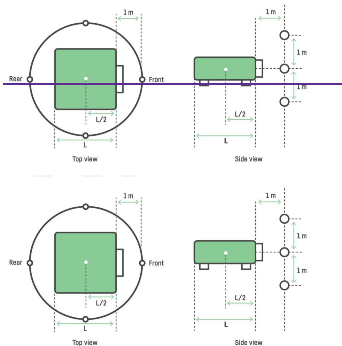
Figure alternating magnetic fields 1. Measurement geometry for the test object.
