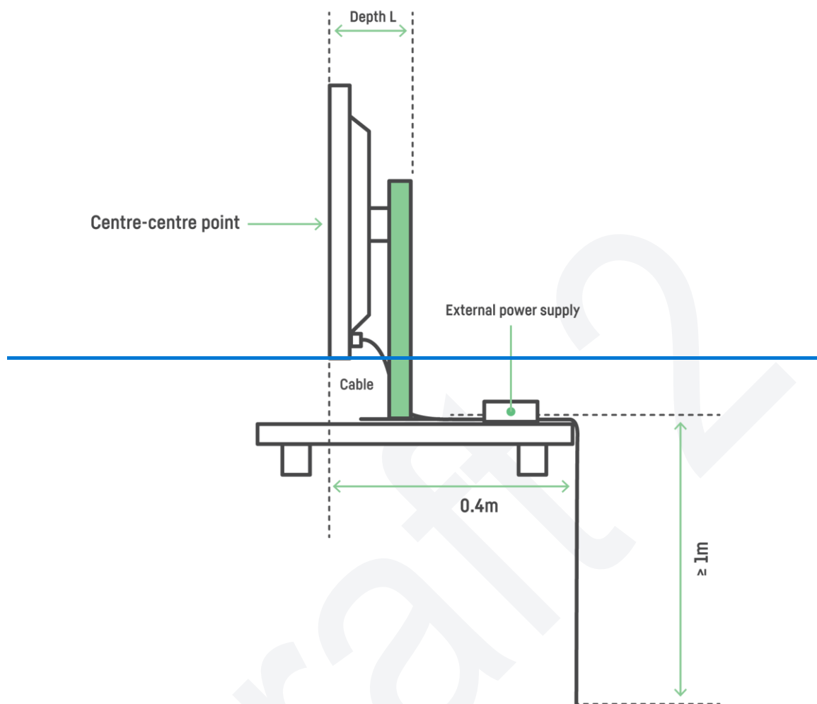
Figure 9.3.3.2. All in one PC with external power supply units.
