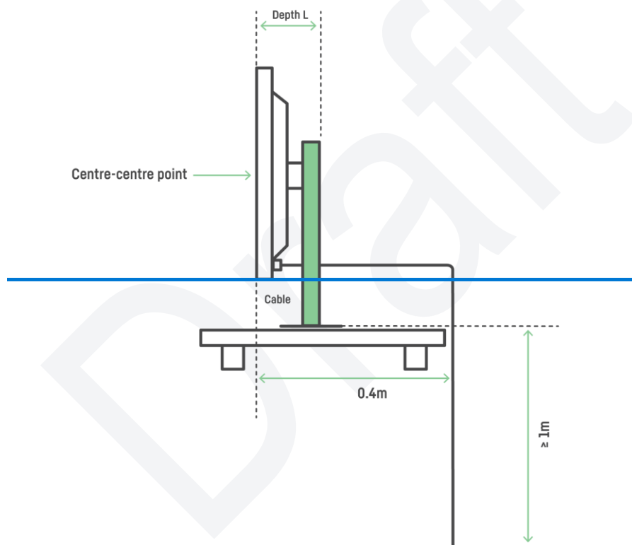
Figure 9.3.3.1. All in one PC without external power supply unit.
