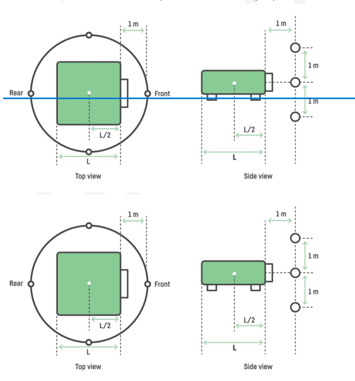
Figure alternating magnetic fields 1. Measurement geometry for the test object.
