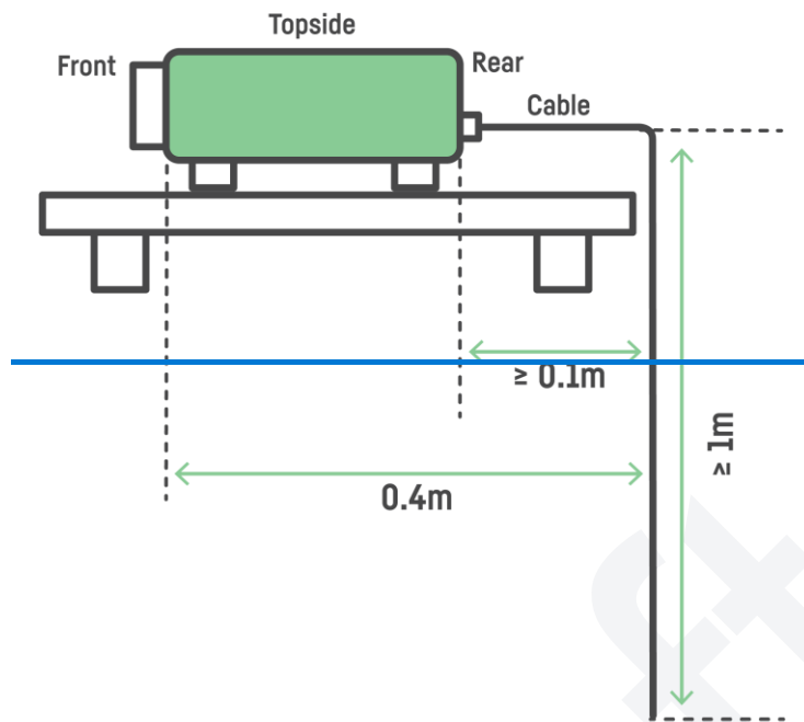
Figure 9.3.3.1. Projector without external power supply unit.
